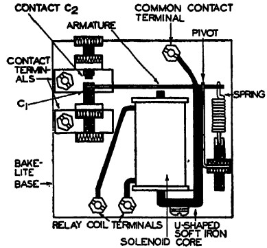
Relay construction.
